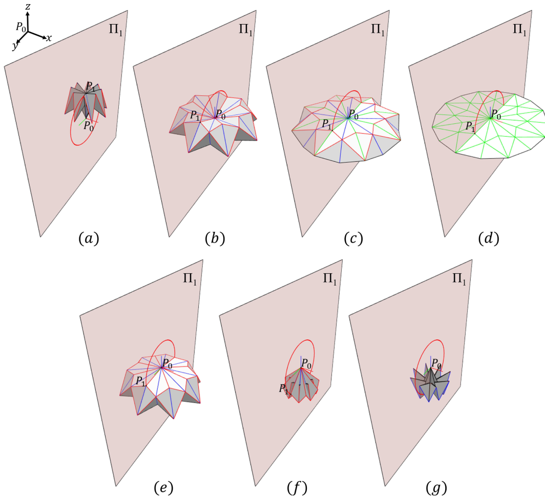
Figure 8: Various origami designs obtained by changing \varphi from 0^\circ to 180^\circ : (a) \varphi = 0^\circ , (b) \varphi = 66^\circ , (c) \varphi = 83^\circ , (d) \varphi = 90^\circ , (e) \varphi = 97^\circ , (f) \varphi = 135^\circ , (g) \varphi = 180^\circ .
