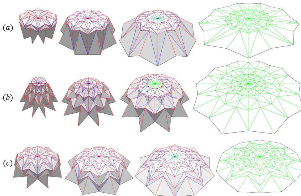
Figure 11: Flat-folding motion.
