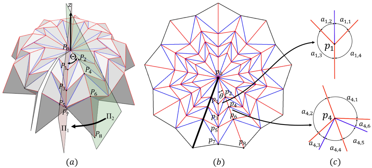
Figure 9: Preparation for along-arc flat-folding.
