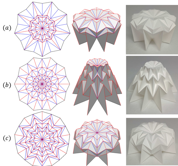
Figure 10: Resulting origami pieces with triangular facets.
