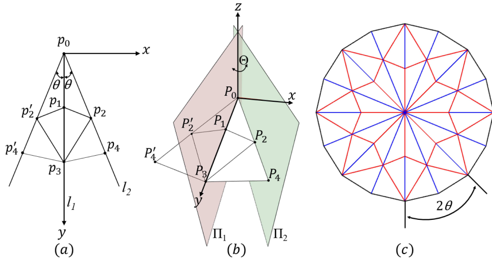
Figure 2: Designing rotationally-symmetric crease pattern consisting of triangular facets.
