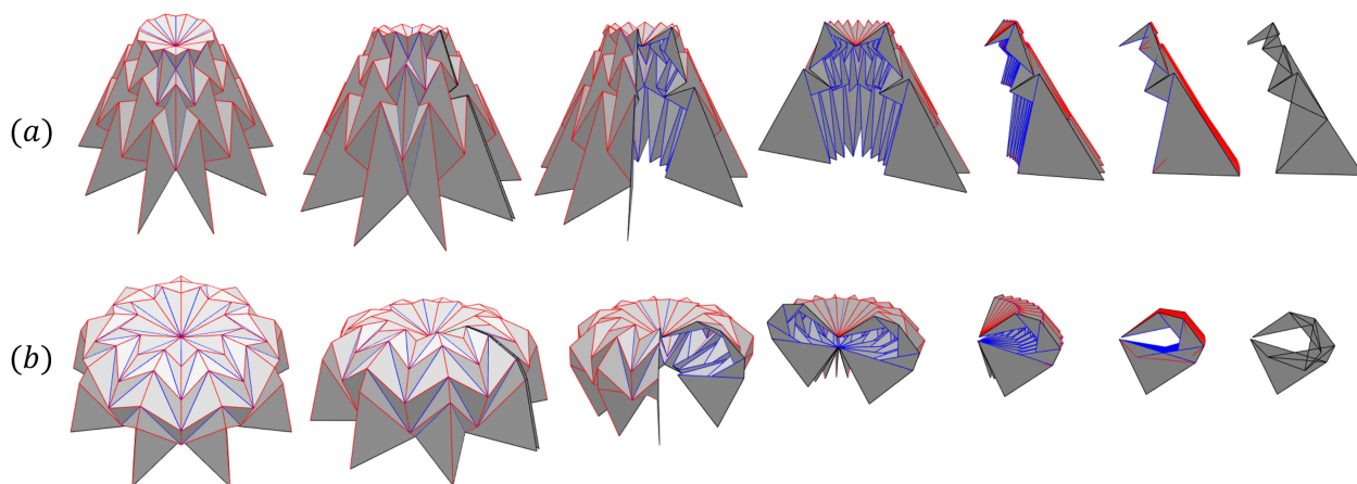
Figure 13: Along-arc flat-folding sequences.
