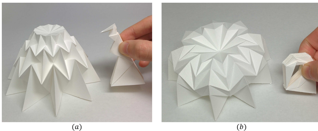
Figure 14: Along-arc flat-folding of real origami pieces.
